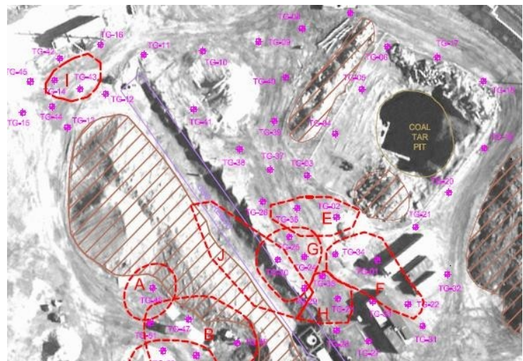
ISCO (Hydrogen Peroxide and Sodium Persulfate) Chemical Treatment areas of the site.
