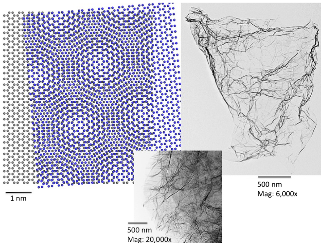
Figure 22. The regular framework structure of graphene sheets overlain upon each other show Moiré patterns, new larger periodic patterns. Image credits—National Institute of Standards and Technology (NIST) and Cabot Corporation (TEM images; http://www.cabot-corp.com/New-Product-Development/Graphenes ).
