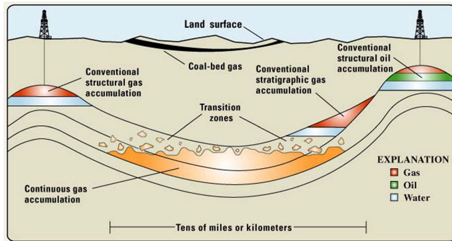
Figure 8. Schematic diagram of the different types of onshore natural gas plays. Conventional resources are buoyancy-driven hydrocarbon accumulations, with secondary migration and structural and/or stratigraphic closures. Unconventional, continuous gas accumulations, in basin centers and transition zones, are controlled by expulsion-driven secondary migration and capillary seal (from U.S. Departments of the Interior, Agriculture, and Energy 2008, p. 46).
